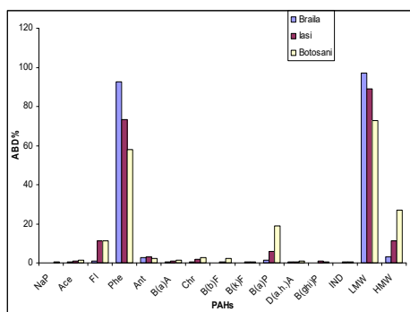
Figure 1. Abundance of individual PAHs, LMW and HMW in analyzed water samples from different areas of the Moldavian Region.
