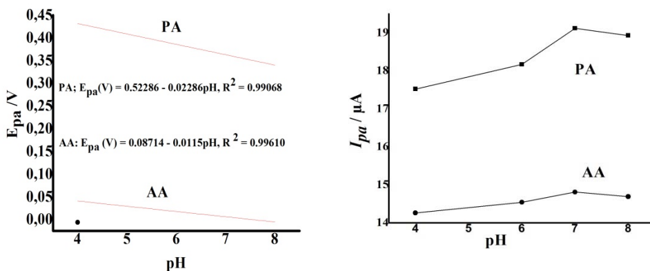
Figure 5. Effect of p\text{H} on the peak potential ( E_p ), Figure 6. Effect of p\text{H} on the peak current ( I_p ), other conditions as Figure 4.
