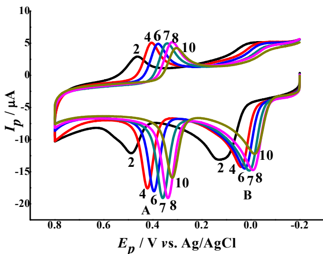
Figure 4. CVs of pH values on the peak current ( I_p ) and peak potential ( E_p ) of 0.1 mM PA (A) and 0.5 mM AA (B) at aGCE, Sensitivity; 100 \mu\text{A/V} .
