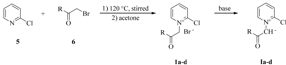
Scheme 2. Synthesis of 1-alkyl-2-chloropyridinium bromides and forming ylides.
