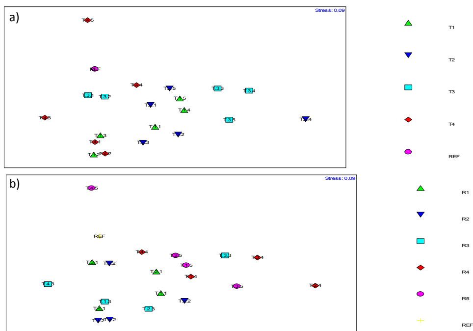
Figure 2. Non metric multidimensional scaling analysis of average metal concentrations in the soils of Ait Ammar mining area, Analysis made “a” by transect, “b” by round
